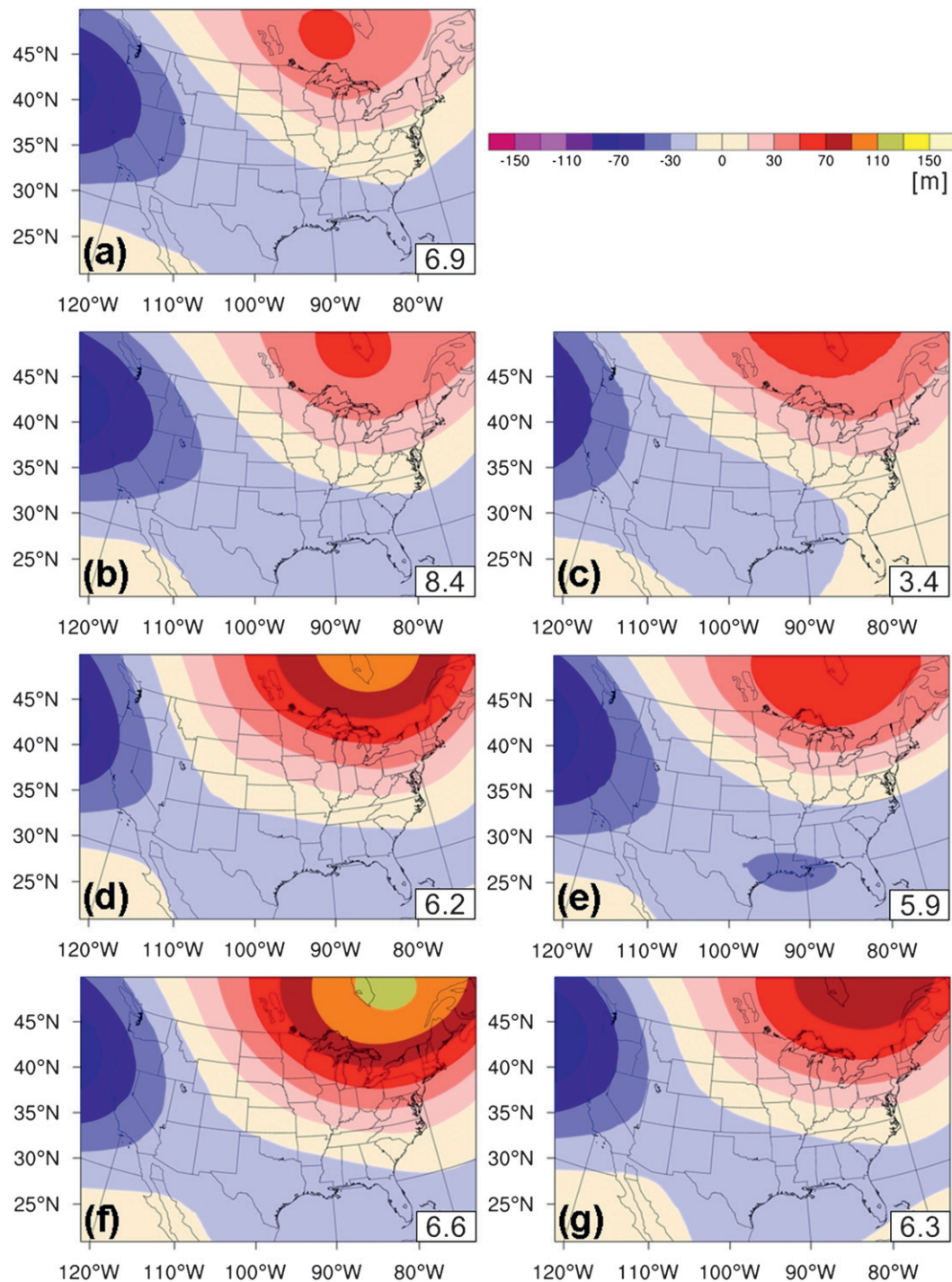
FIG. 3. Composite 500-hPa height anomalies for top 10% of Coastal CA monthly precipitation extremes: (a) NARR, (b) ECPC, (c) HRM3, (d) MMSI, (e) CRCM, (f) RCM3, and (g) WRFP. Contour scale for all plots is in the upper right. Insets on the lower right of each panel give the average precipitation for the top 10% extremes, with UW precipitation in (a). Contours are in meters, and precipitation is in \text{mm day}^{-1} .
