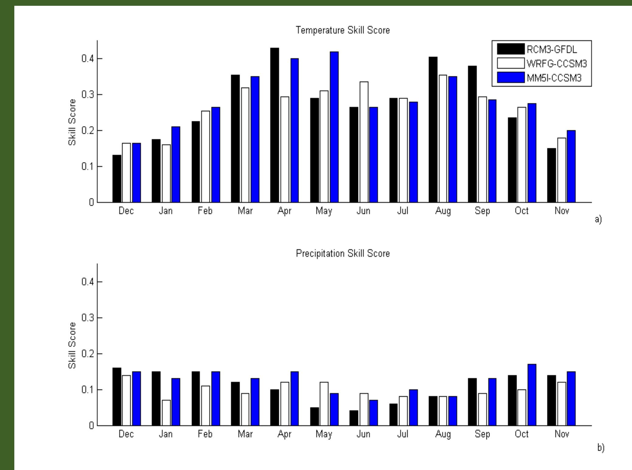
Figure 1: Monthly skill scores for RCM3-GFDL, WRFG-CCSM3, and MM5I-CCSM3 regional climate models (a) temperature and (b) precipitation for the period 1970-1999 for the Southeast U.S.
