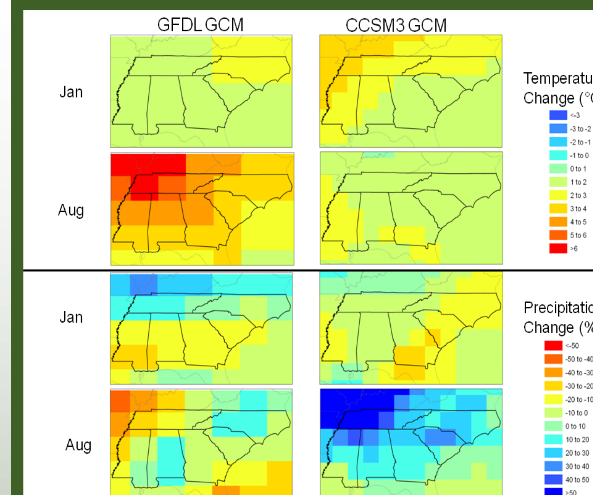
Figure 3: January and August temperature and precipitation change projections from two GCMs (100km resolution) used in NARCCAP. These were used as boundary conditions for RCMs in Figure 4 for the period 1970-1999 to 2041-2070.
