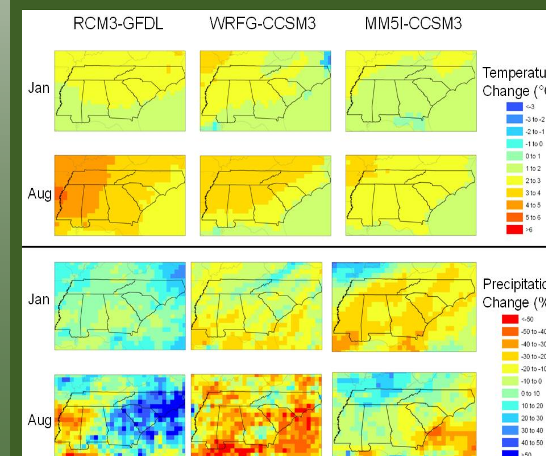
Figure 4: January and August temperature and precipitation change projections from three NARCCAP RCMs for the period 1970-1999 to 2041-2070.
