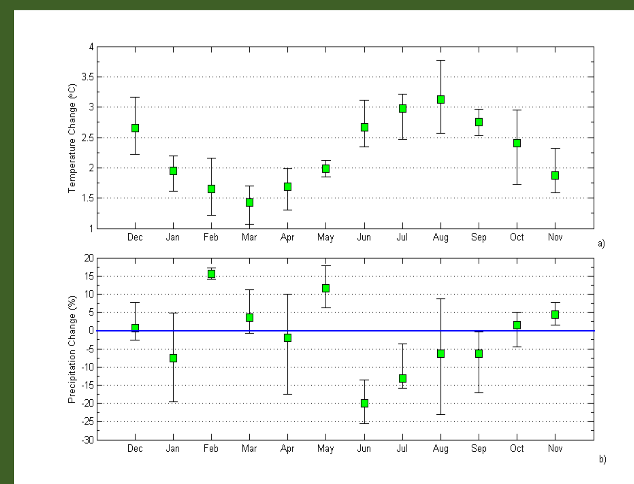
Figure 2: Projected (a) temperature and (b) precipitation change for the Southeast U.S. from 1970-1999 to 2041-2070. Green boxes represent weighted average of three RCMs. Error bars represent lowest and highest individual model mean.
